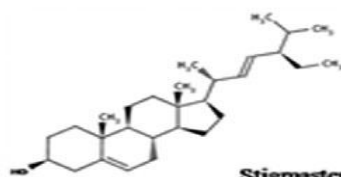
Stigmasterol
