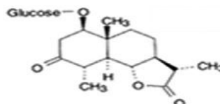
Taraxacolid-β-D-glucoside
